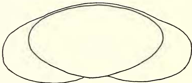
TEXT-FIG. 8. Alisporites circulicarpus sp. nov. Diagrammatic reconstructions. A, Proximal polar aspect. B, Polar section. \times 1,000 .
